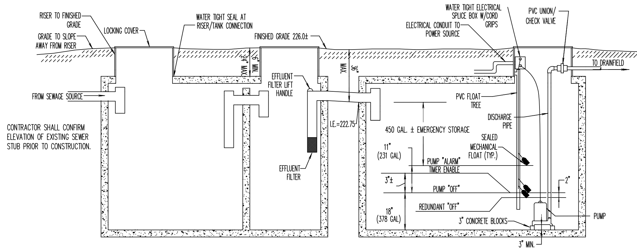
1,000 GALLON SEPTIC TANK DETAIL (NOT TO SCALE)
