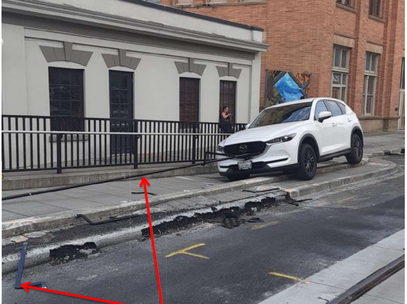
Railing forced forward/posts broke away at railing/post (weld) and post/curb connections.
