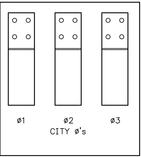
DETAIL "A" PHYSICAL PHASE ARRANGEMENT AS VIEWED FROM REAR COMPARTMENT
