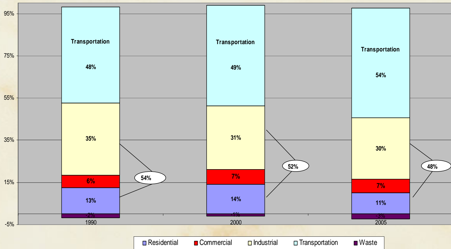
Community Emissions 1990-2005
