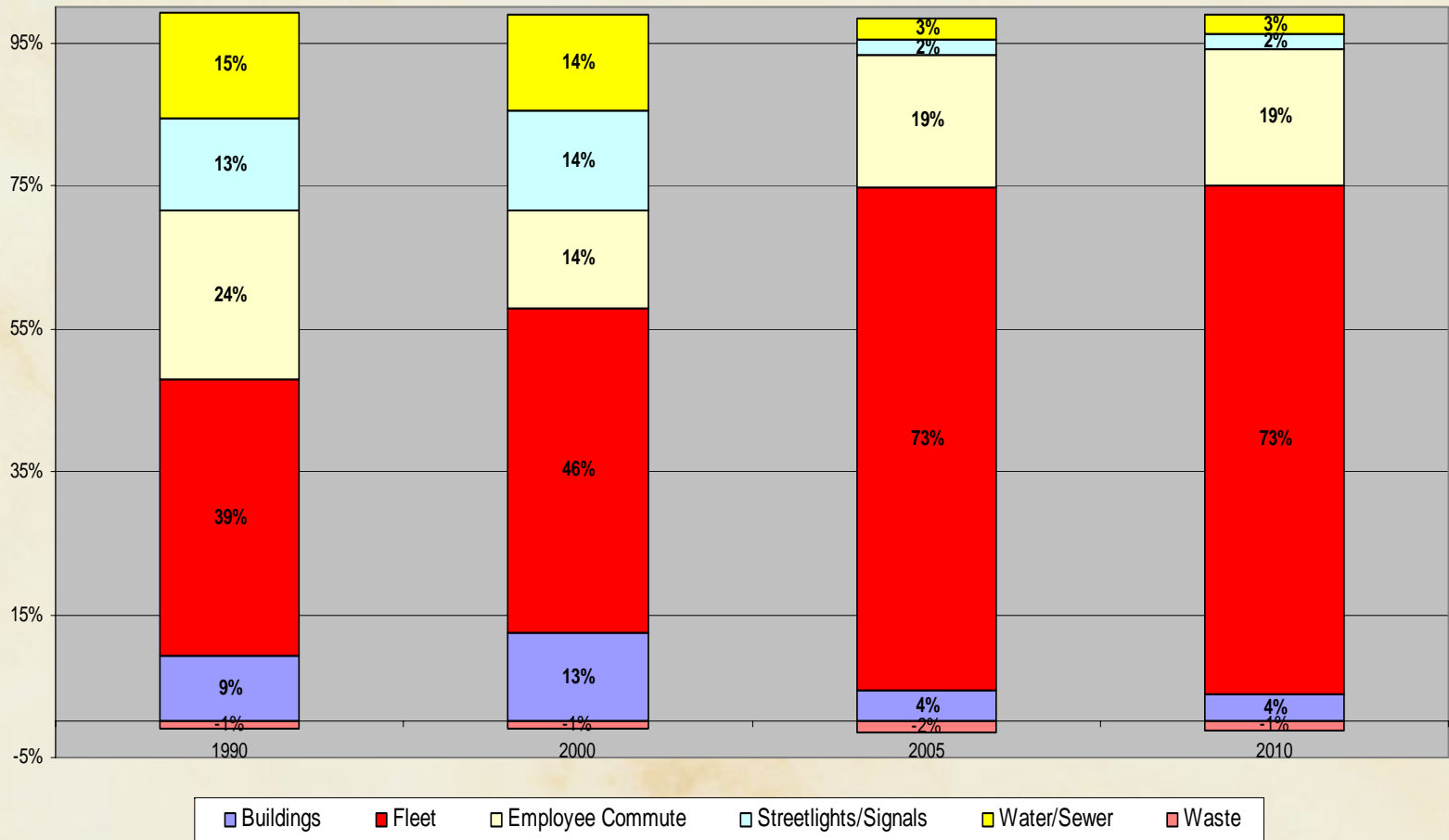
Government Emissions 1990-2010
